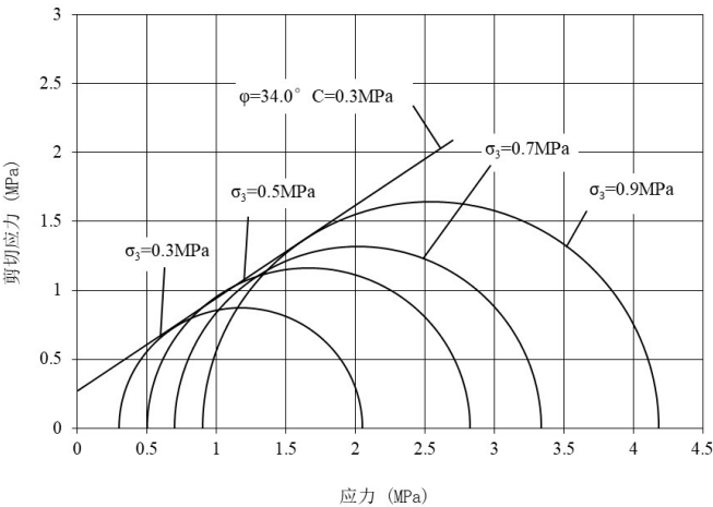
图4 莫尔圆和剪切破坏强度线 Fig. 4 Mohr's Circle and Shear Strength Envelope
